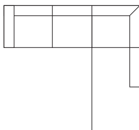
Corner Sofa Right Size: 297 x 222 x 89 cm Seat depth: 50 cm Seat height: 45 cm
