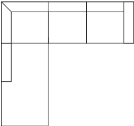
Corner Sofa Left Size: 295 x 106/240 x 68 cm Seat depth: 64/198 cm Seat height: 44 cm
